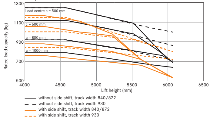
Basic capacities RX 50-13 triplex mast, SE tyres
