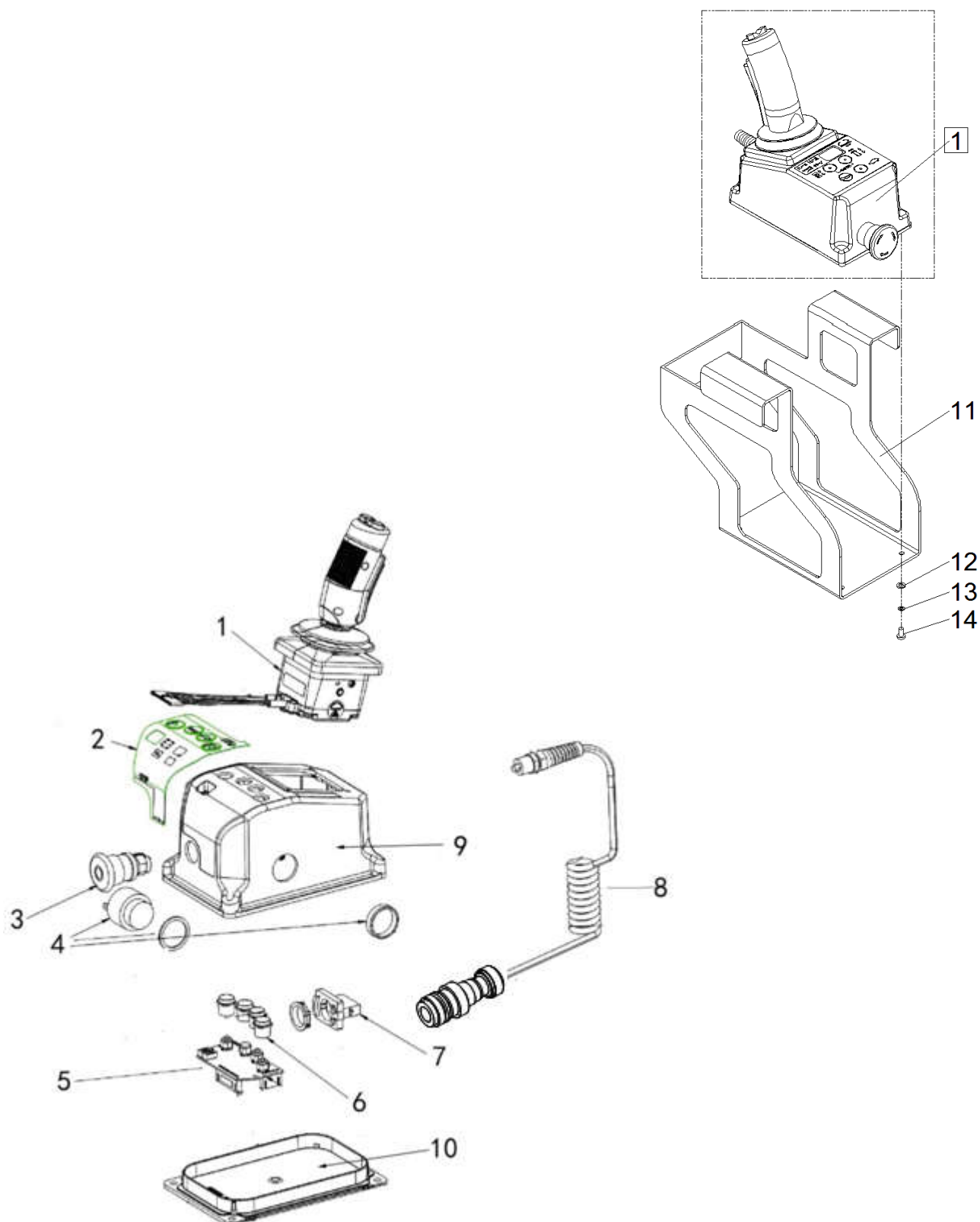
Figure 13 Platform controller components
