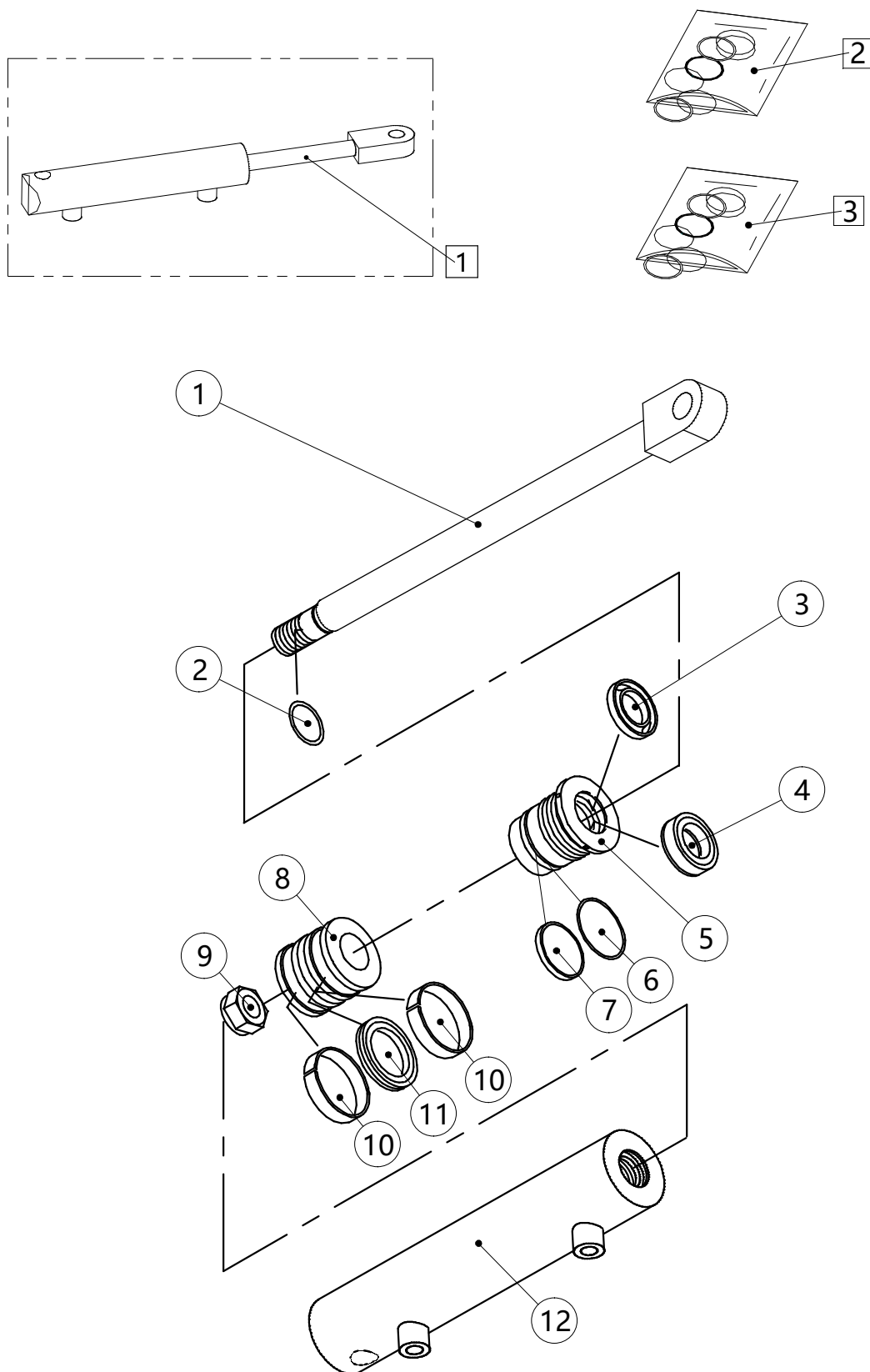
Figure 19 Steering Cylinder
