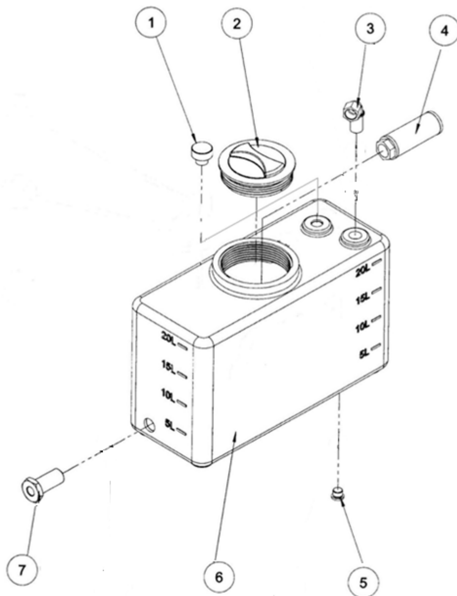
Figure 20 Hydraulic oil tank
