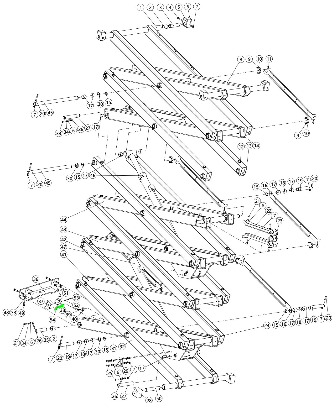
Figure 9 Parts and components of scissors (SC14H/SC14E)
