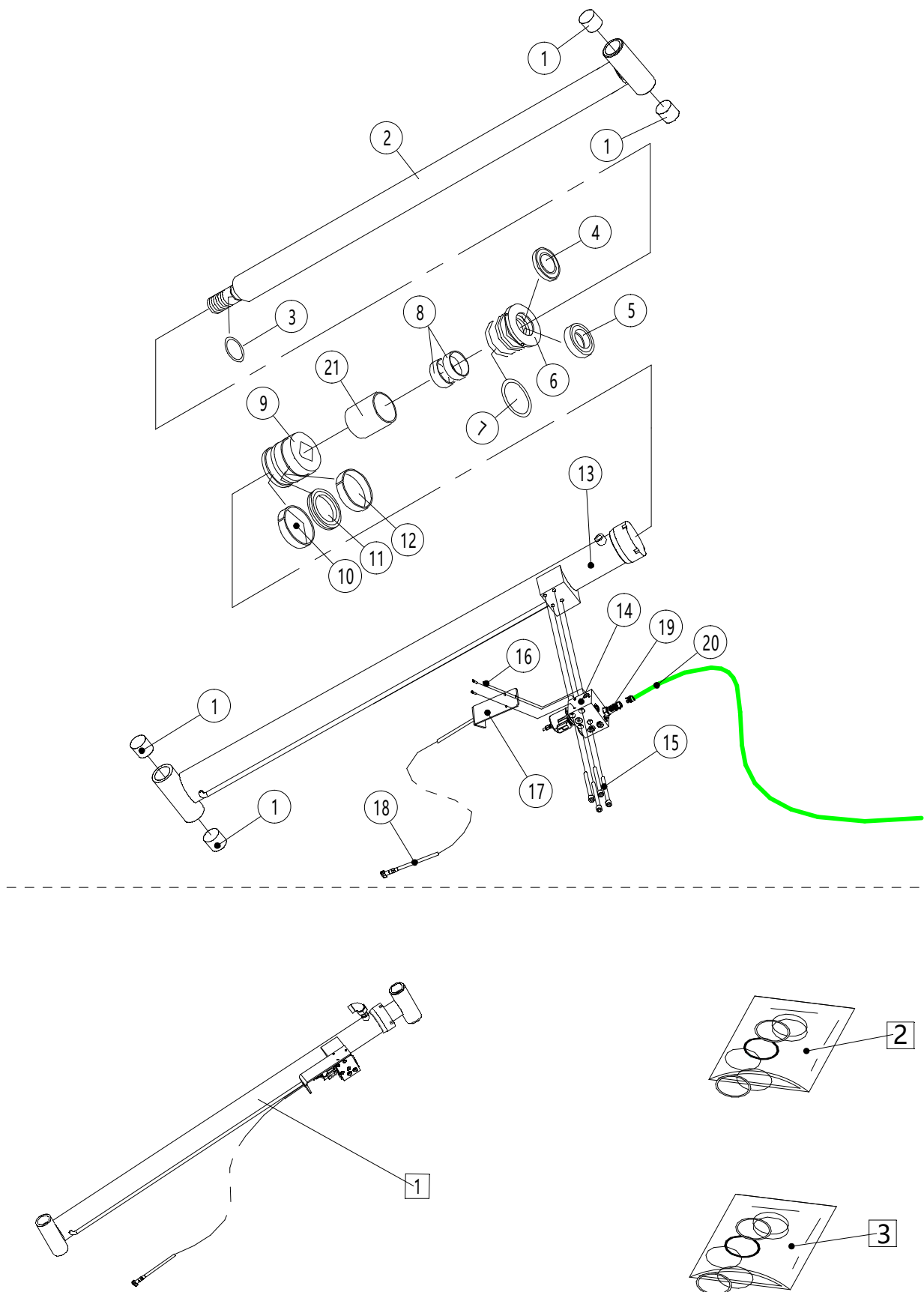
Figure 17 Cylinder
