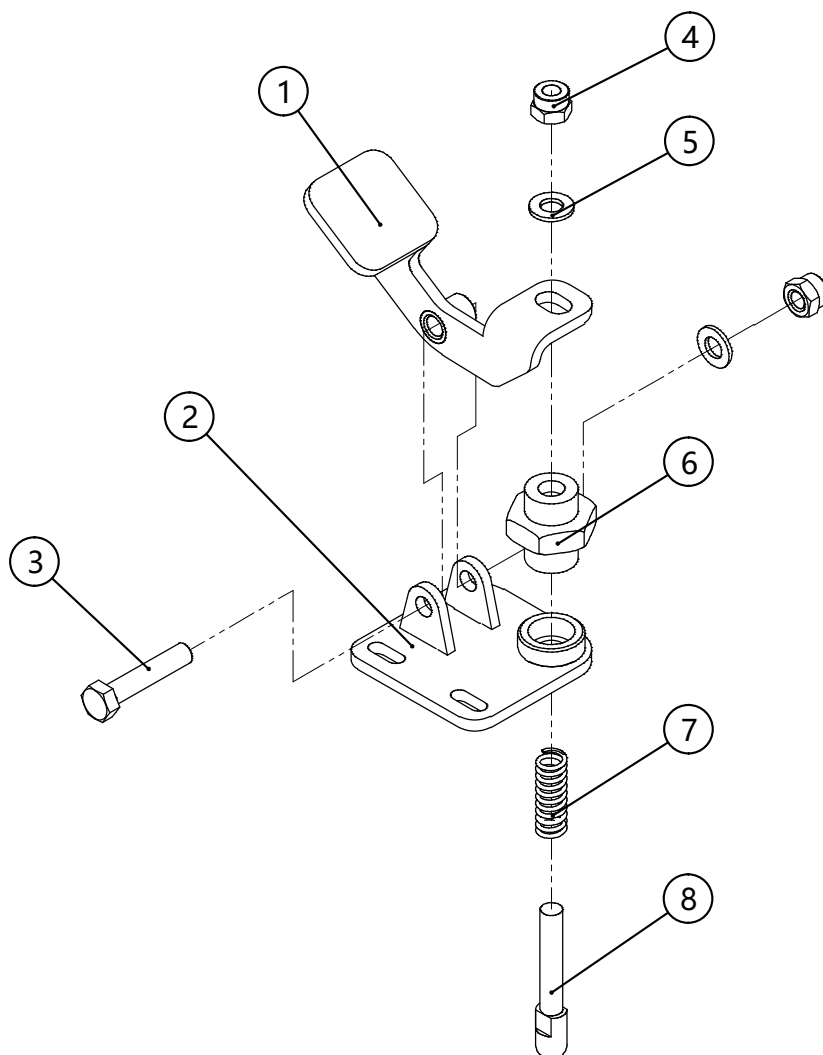
Figure 14 Pedal lock
