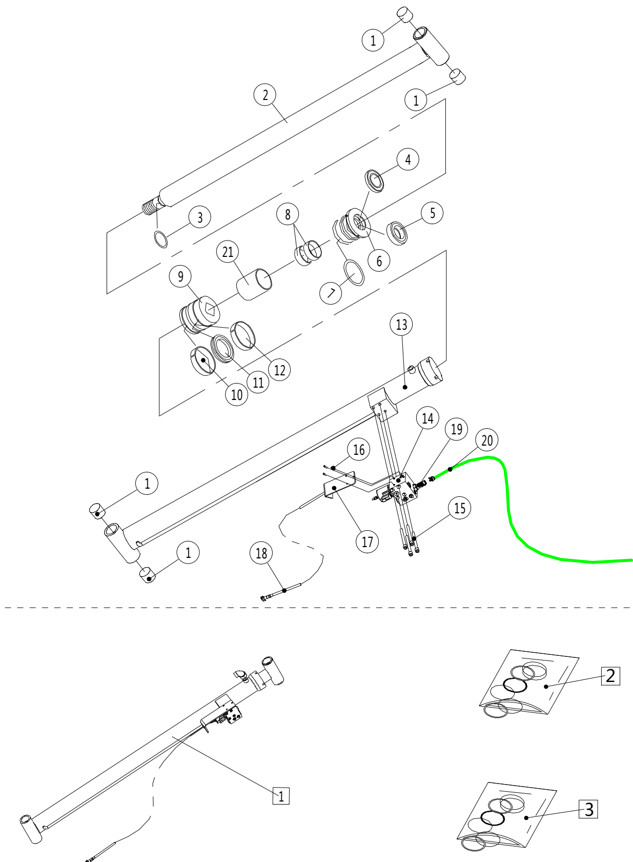
Figure 15.1 Cylinder (SC16H)
