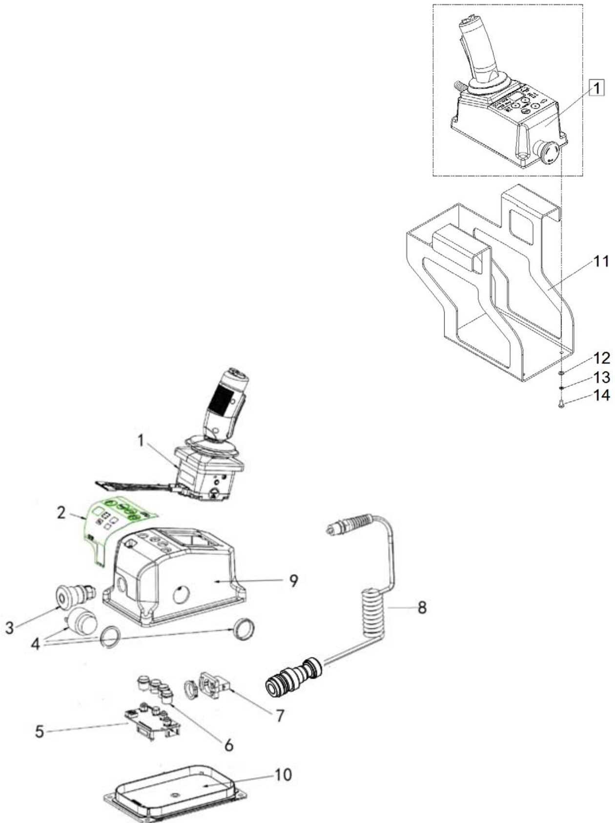
Figure 11.1 Platform controller components
